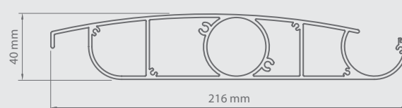
Blade cross-section
