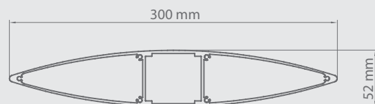
Blade cross-section
